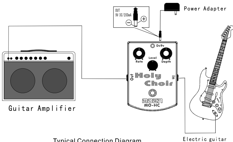
Typical Connection Diagram
